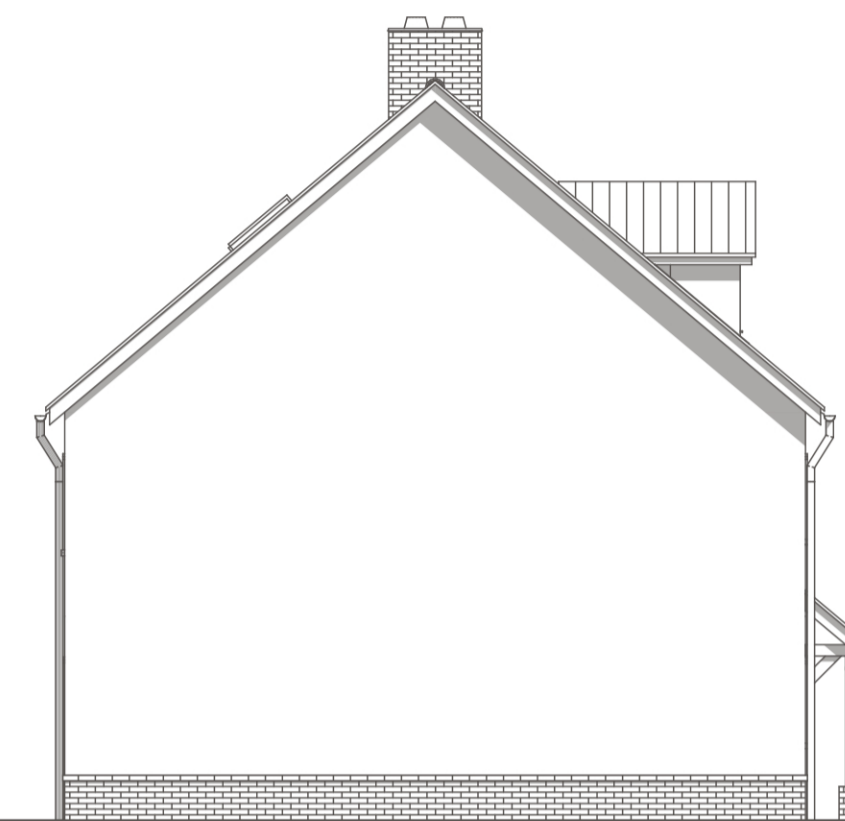
SIDE ELEVATION
