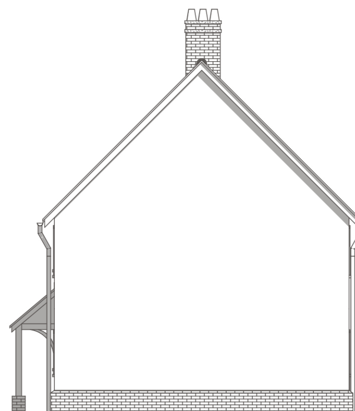
SIDE ELEVATION
