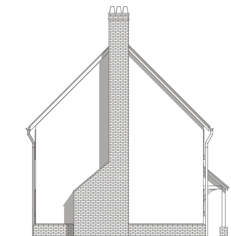
SIDE ELEVATION
