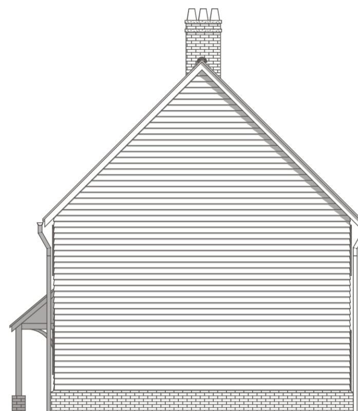
SIDE ELEVATION
