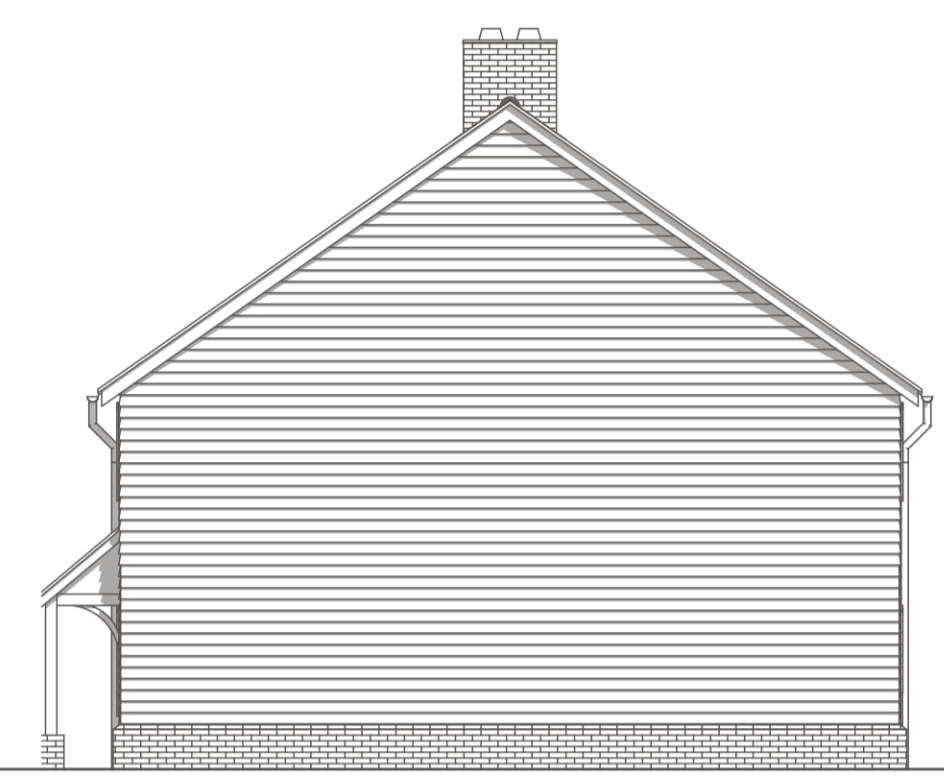
SIDE ELEVATION
