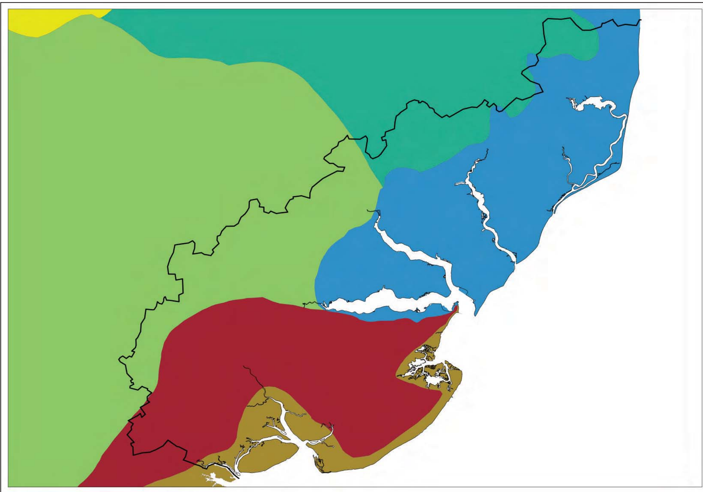
Figure 04 Countryside character
